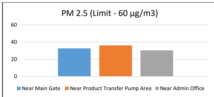
Figure 2: Graphical representation of average trend of PM 2.5 in µg/m 3
