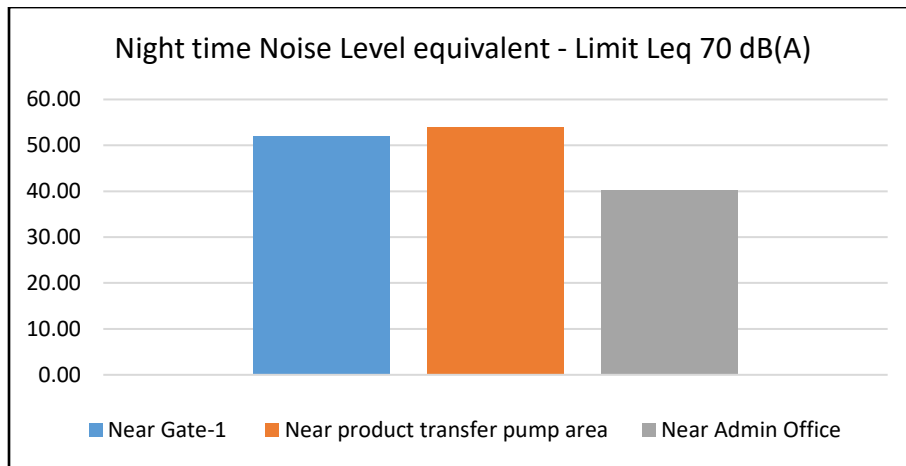
Figure 6: Graphical representation of Noise Level in Leq dB(A) in the Night-time
