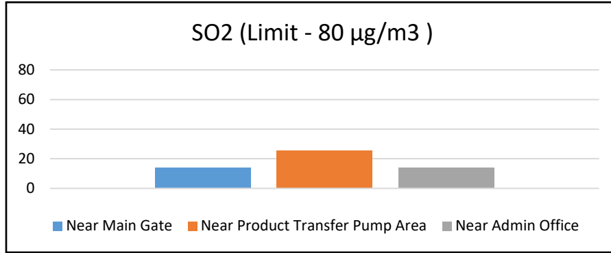
Figure 3: Graphical representation of average trend of SO 2 in in µg/m 3
