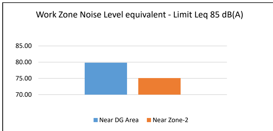
Figure 10: Graphical representation of trend of Work Zone Noise Level in Leq dB(A)
