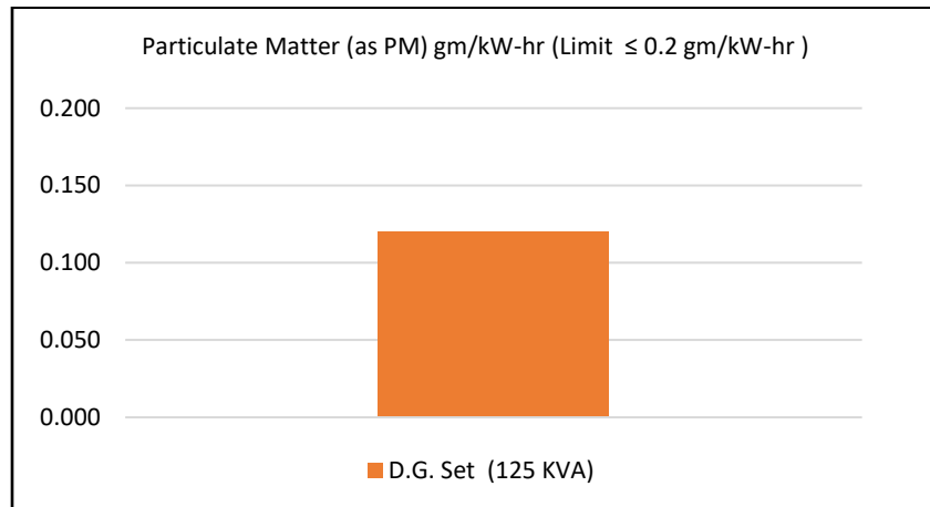
Figure 7: Graphical representation of average emission of Particulate Matter in g/kW-hr
