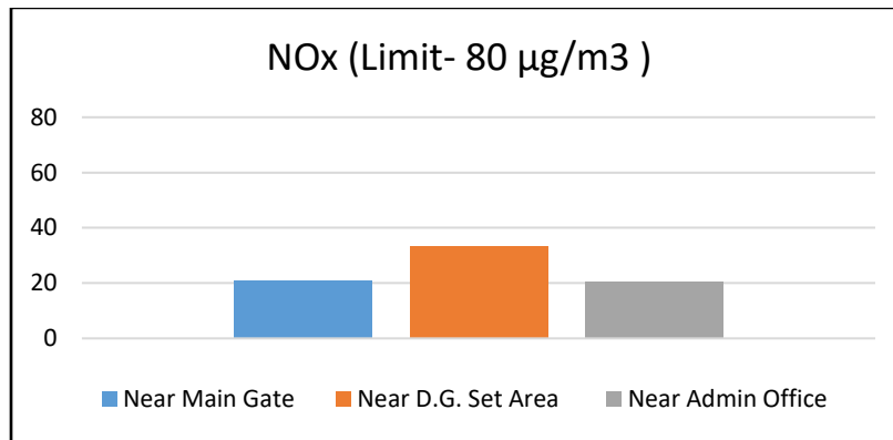
Figure 4: Graphical representation of average trend of NO x in in µg/m 3
