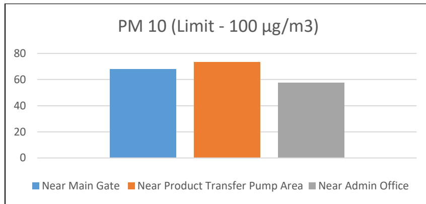
Figure 1: Graphical representation of average trend of PM 10 in µg/m 3
